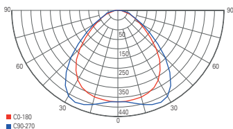
light distribution curve 100072
