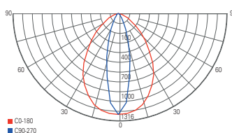
light distribution curve 732107
