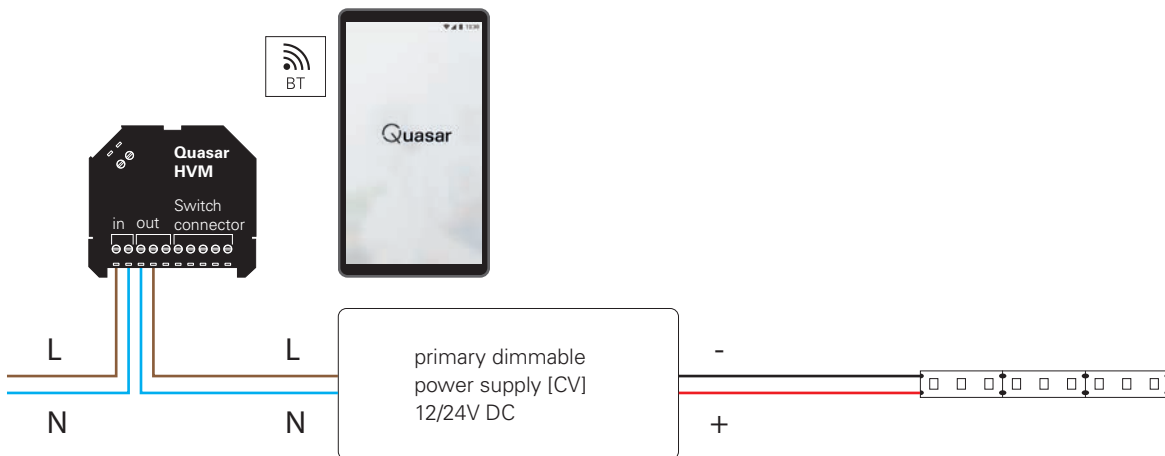
Quasar HVM [843007] S. 939 matching power supplies p. 904-905
