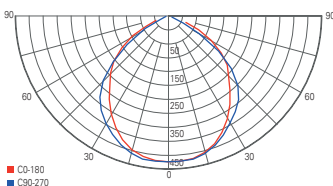
light distribution curve 707032
