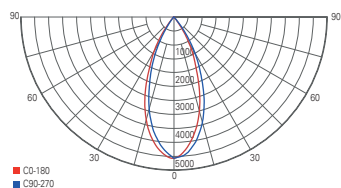
light distribution curve 707106 | 707107
