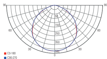
light distribution curve 732102
