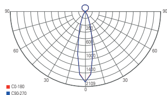
light distribution curve 620111
