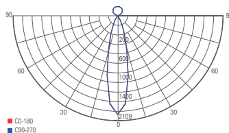
light distribution curve 620114
