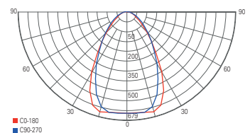
light distribution curve WW | 72W
