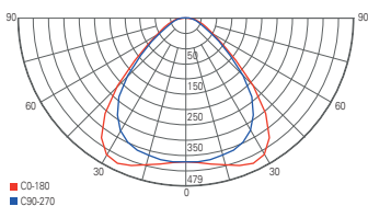
light distribution curve 100069
