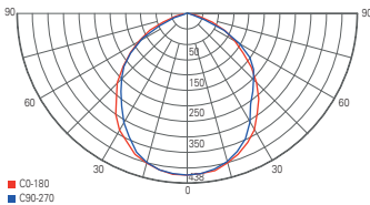
light distribution curve 707030
