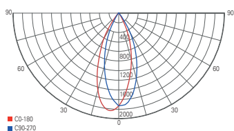
light distribution curve 707098 | 707099
