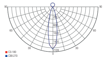
light distribution curve 620117
