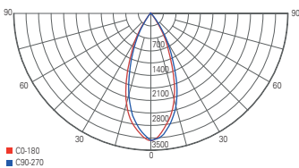
light distribution curve 707102 | 707103
