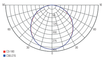
light distribution curve 100044
