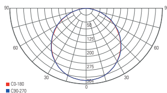
light distribution curve 100045
