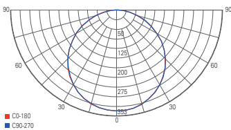
light distribution curve 100032
