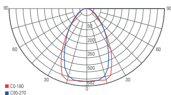
light distribution curve WW | 45W
