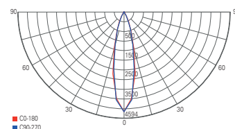
light distribution curve 620105
