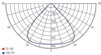
light distribution curve HIGHBAY NORMAE with lens 90°
