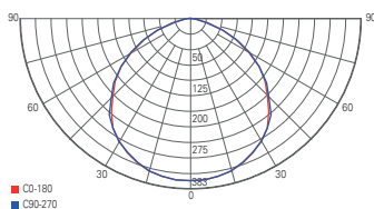
light distribution curve 732103
