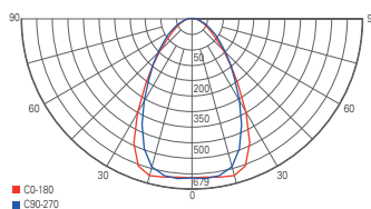
light distribution curve WW | 55W
