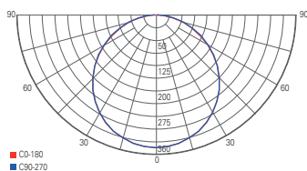
light distribution curve 100051
