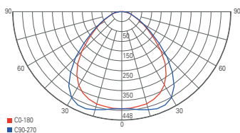
light distribution curve 100059
