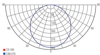
light distribution curve 100056
