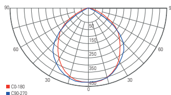
light distribution curve 707033
