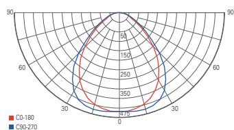
light distribution curve 100046
