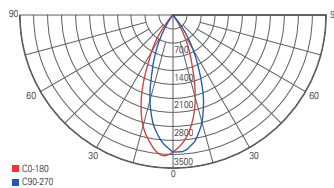
light distribution curve 707104 | 707105
