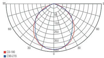
light distribution curve 707031
