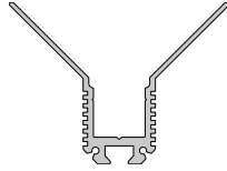
dry construction profile inside corner page 766
