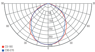
light distribution curve 732027
