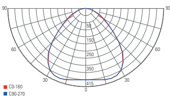
light distribution curve 100058
