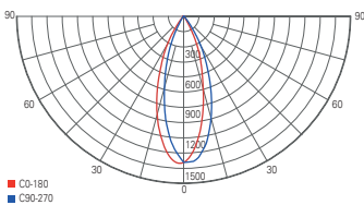
light distribution curve 707094 | 707095
