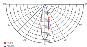
light distribution curve 620107
