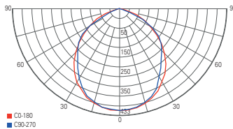
light distribution curve 732028
