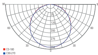
light distribution curve 565221
