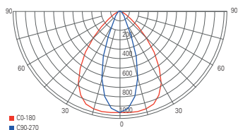
light distribution curve HIGHBAY NORMAE with lens 30°/70°
