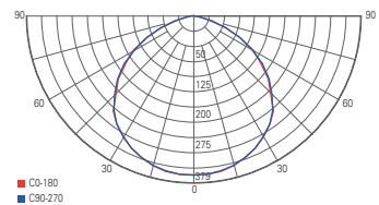
light distribution curve 732101
