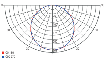
light distribution curve 100076
