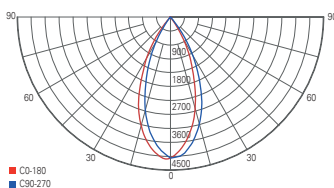
light distribution curve 707108 | 707109
