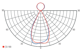
light distribution curve
