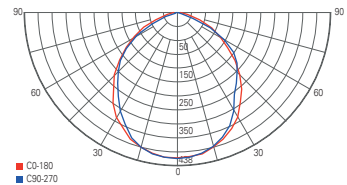
light distribution curve 732029
