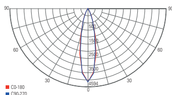
light distribution curve 620106
