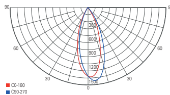
light distribution curve 707096 | 707094
