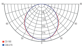
light distribution curve 100047
