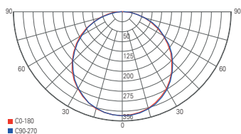
light distribution curve 100035
