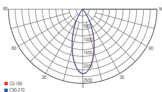
light distribution curve 707100 | 707101
