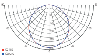
light distribution curve 100057
