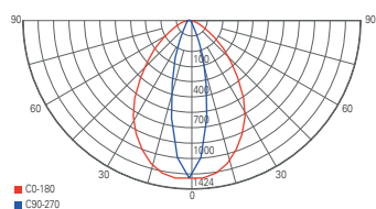
light distribution curve 732106
