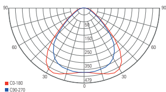
light distribution curve 100043
